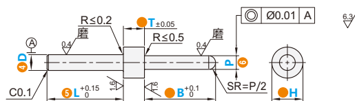
球面型 DAVHKR DAVHS
