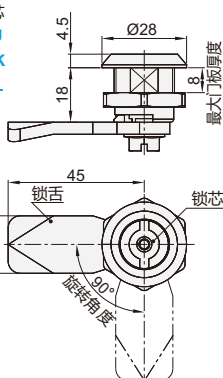
双牙形锁芯 GAAXSEJ GAAXSEK GAAXSEL
