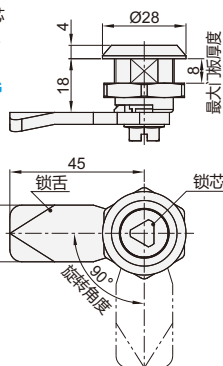
三角形锁芯 GAAXSEE GAAXSEF GAAXSEG
