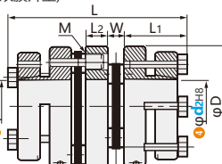
CADHP (双膜片型)
