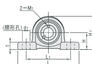
BADRCP (简易轴台型)
